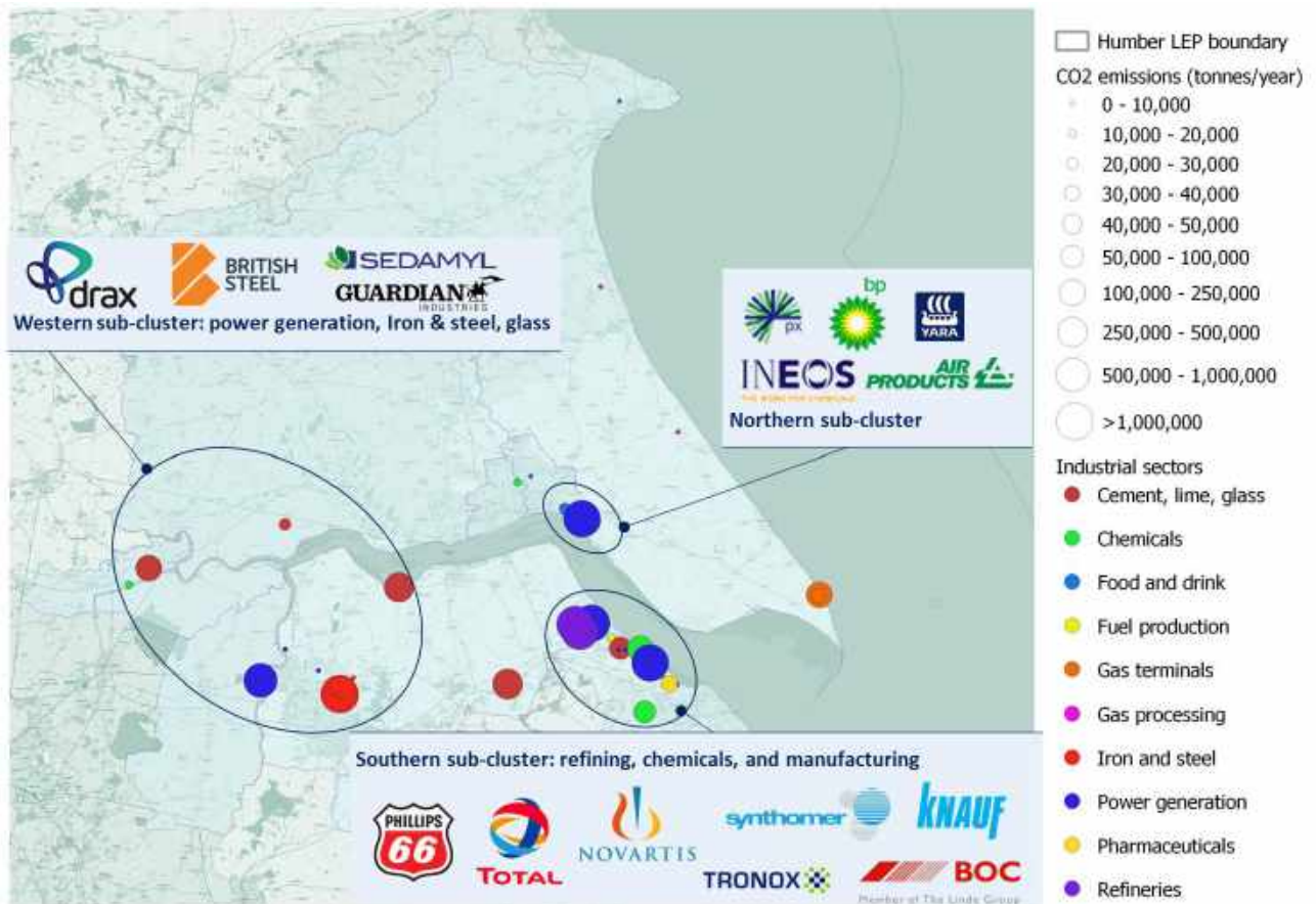
Figure 6: Overview of the main emitters within the Humber and emissions sub-clusters
